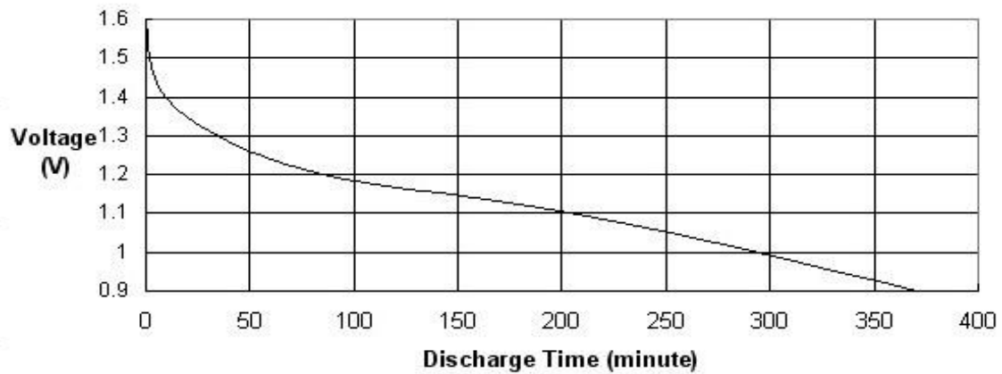
3.9Ω Continuous Discharge Curve
