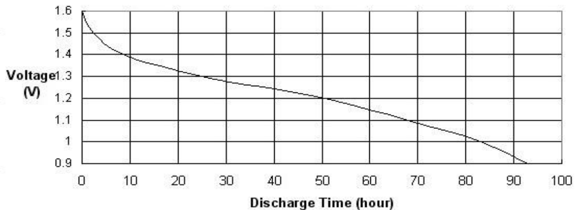
43Ω 4hour/day Discharge Curve
