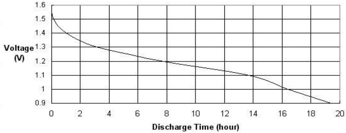
10Ω Continuous Discharge Curve
