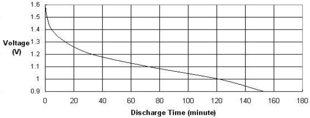
3.9Ω Continuous Discharge Curve
