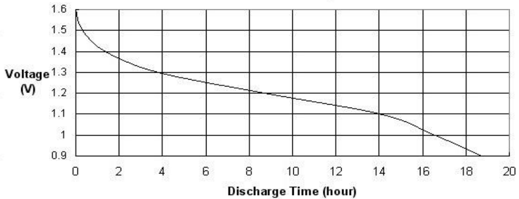
20Ω Continuous Discharge Curve
