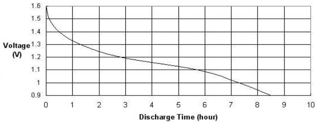
10Ω Continuous Discharge Curve
